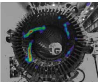
Measurement during a high voltage test
